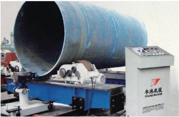
防窜动滚轮架 Anti-scurrying turning-rolls
