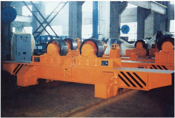
160T行走式滚轮架 160T The traveling trolley turning-rolls
