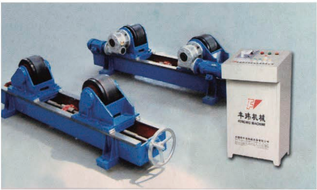
丝杠可调式滚轮架 Conventional power control turning-rolls
